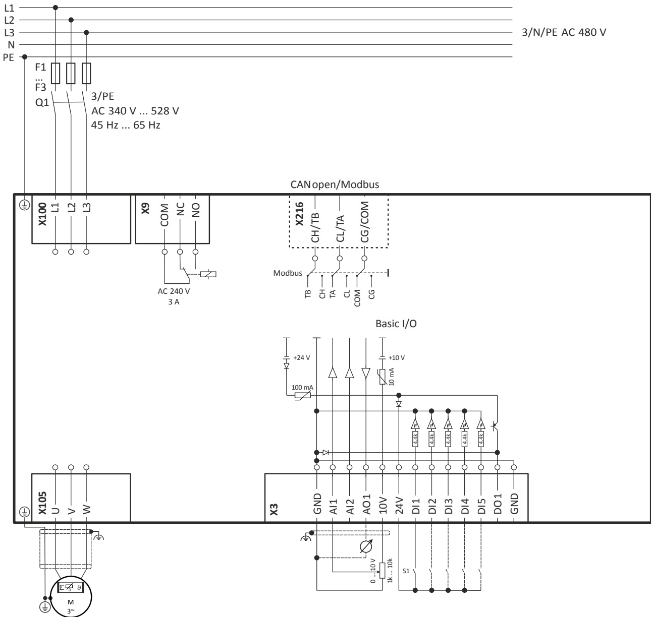
Fig. 8: Wiring example
