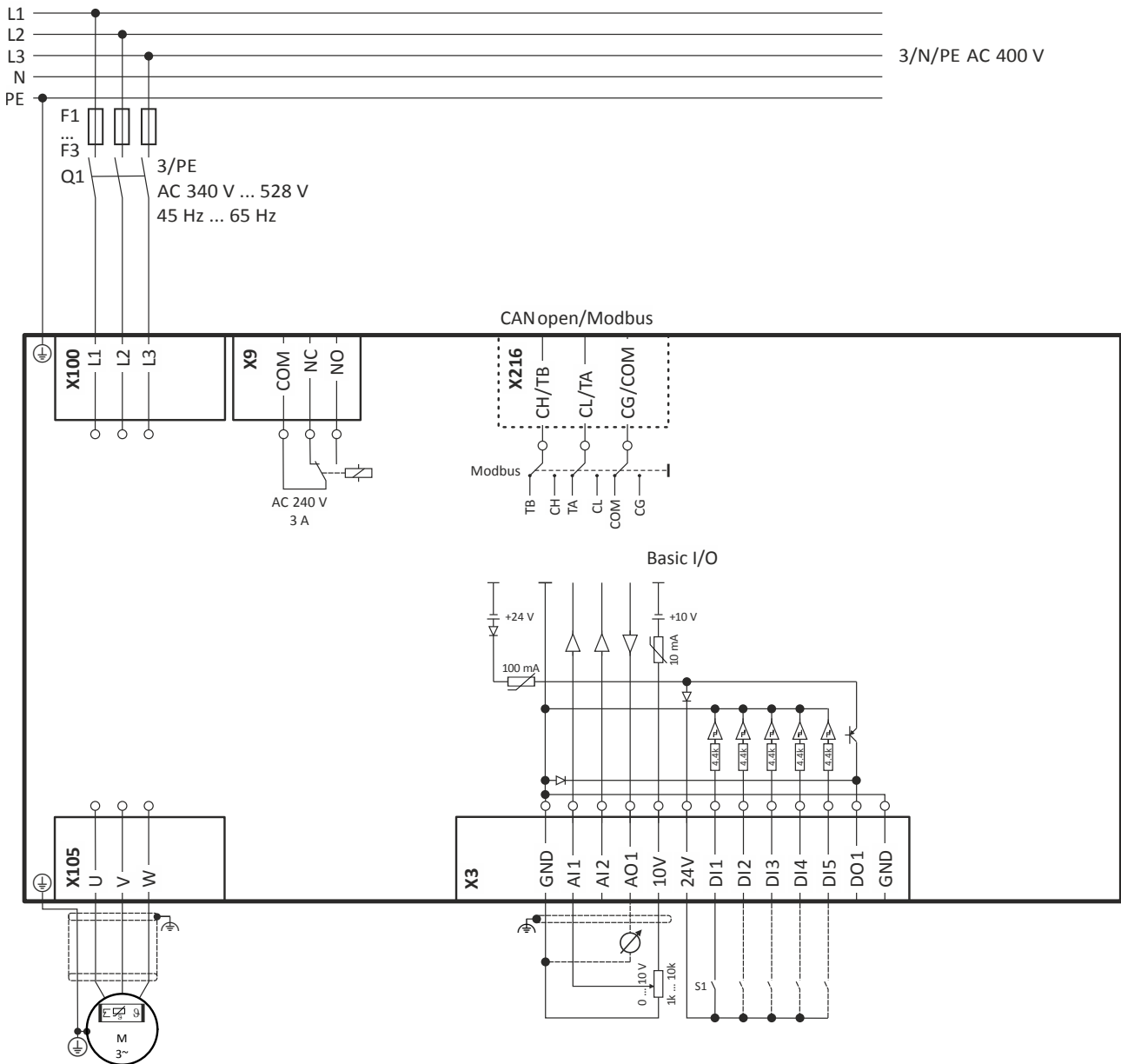
Fig. 7: Wiring example
