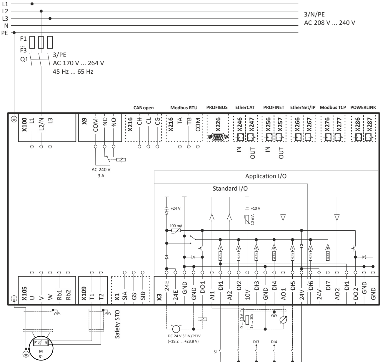
Fig. 7: Wiring example
