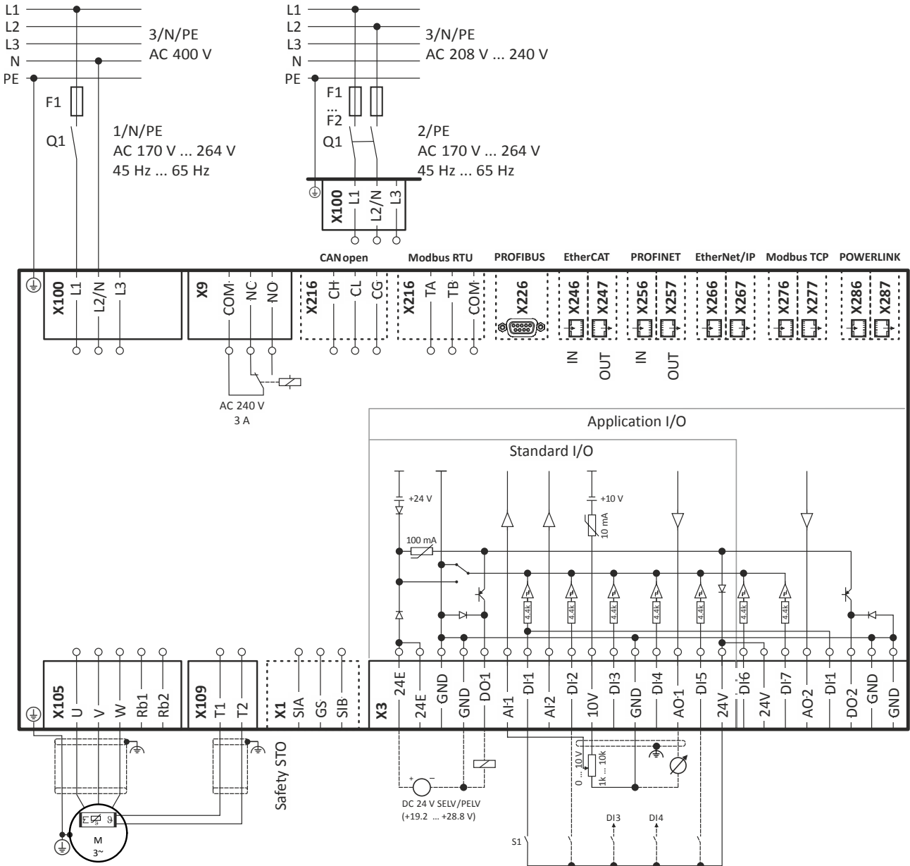
Fig. 5: Wiring example
